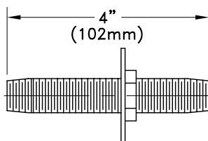
3/8" IPS MOUNTING SHANKS WITH LOCKNUTS AND WASHERS
